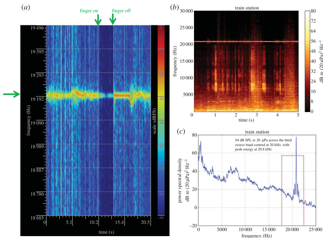
Figure 1. Acoustic field measurements taken by (a) an iPhone 5 S in a public library (the horizontal arrow indicating the main tone at approx. 19.2 kHz) and (b) a calibrated microphone in a railway station. (a) The temporary placement of the author's finger over the microphone (as indicated by the vertical arrows) allows the signal to be confirmed as acoustic and not electromagnetic pickup (see appendix A). Spectrograms (a,b) plot how the distribution of energy across frequencies varies in time. These data can be summed over time to produce the power spectral density (PSD, as shown in (c) for the data in (b)). The sound pressure levels are calibrated in (b,c) and traceable back to primary standards, but not in (a). Fluctuations in frequency in (a) are probably Doppler and diffraction effects as the phone is moved into position. The vertical dashed lines in (c) show the upper and lower frequency limits of the third-octave band centred on 20 kHz, and the horizontal dashed (red) line shows the level of broadband signal that would give the same third-octave SPL as the measured ultrasonic signal. See appendix A for details on instrumentation.
