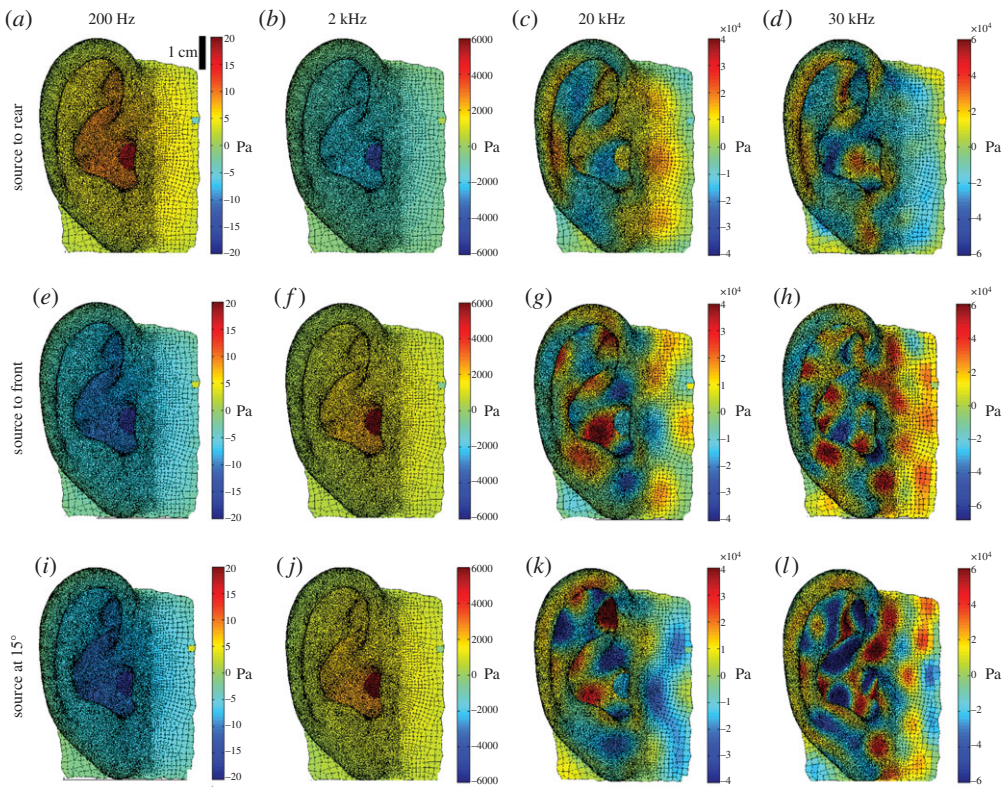
Figure 6. The real part of the scattered pressure (in Pascal) from a point source placed 1 m from the opening of the ear canal, and in the same horizontal plane as it (calculated using boundary element method optimized for high performance computing after the manner of Grace et al. [89]). (a–d) When the source is directly behind the ear, (e–h) when the source is directly in front of the ear, (i–l) when the source is angled 15^\circ outwards, away from the front position. The columns from left to right are for increasing source frequency: 200 Hz (a,e); 2 kHz (b,f); 20 kHz (c,g); 30 kHz (d,h). The point source has a volume velocity amplitude of 1 \text{ m}^3 \text{ s}^{-1} for all plots, and this causes the acoustic pressure naturally to increase with frequency (because there is a scaling factor between them that is proportional to frequency). For simplicity the flesh is assumed to be acoustically rigid. The geometry of the pinna was adapted from Kahana & Nelson [90] with an added ear canal depth of 2.5 cm. The ear canal in this model is straight so that the eardrum is visible in every image at the base of the ear canal. Human ear canals contain a bend, although in some individuals this is less pronounced than in others.
