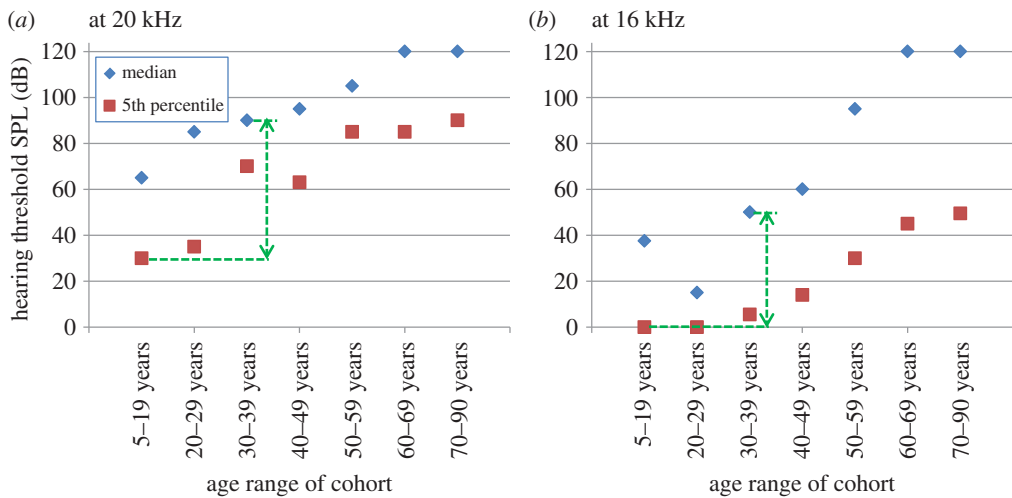
Figure 4. The hearing threshold (pure tone audiometry) as a function of age, showing median and 5th percentile. Data taken from Rodríguez Valiente et al. [10], who used a total dataset of 645 people. Data at 0 dB and 120 dB re 20 \mu Pa have been influenced by the threshold and saturation limits of the instrumentation and so contribute less reliably to the statistics. The vertical arrows indicate the difference between the median in the 30–39 age group, and the 5th percentile in the 5–19 age group.
